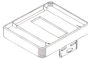
← Cover ( Polypropylene +Polyamide/Glass Fiber )
